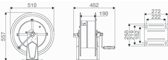
HM 610 - Dimensions in mm
