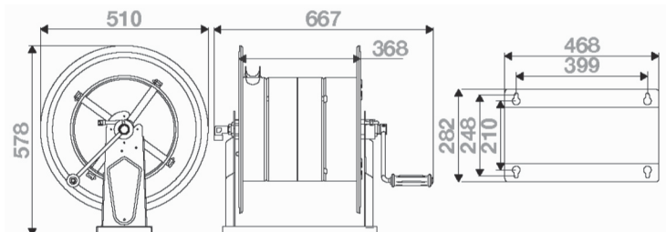
HM 710 - Dimensions in mm
